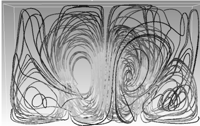
Fig. 3. Streamlines starting from mixer plane (rpm:900 min -1 )
